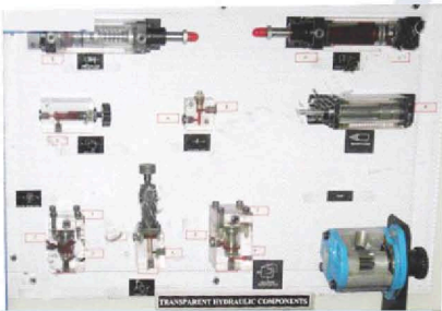
Cut Section of Hydraulic Components
