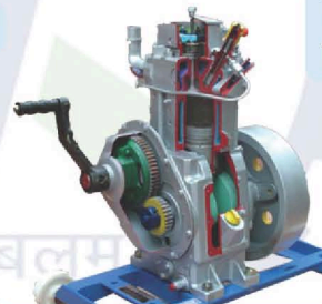
Diesel Engine Cut Section Running Condition Stationary Type
