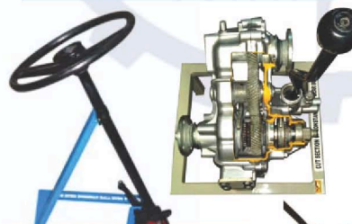
Steering System Worm and Roller Type
